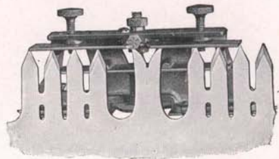
Fig. 6—GRADUATED GAUGE
